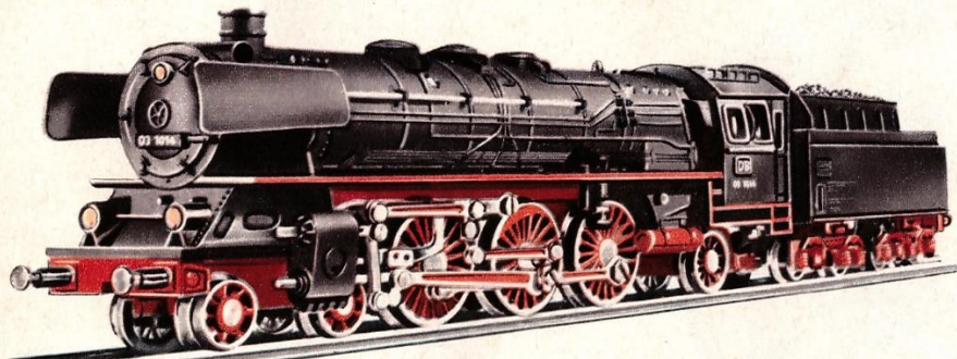
01165 4-6-2 Express Locomotive with Tender Exact scale model of 4-6-2 heavy express locomotive Series 03 of the German Federal Railways, with four-axle Tender. Overall length: 8.5"
